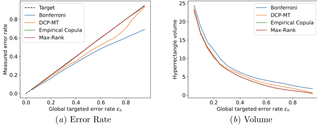
Figure 19: Multi-tests methods' mean error rates and volumes for the music origin (Zhou et al., 2014) data set.
