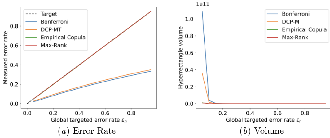
Figure 28: Multi-tests methods' mean error rates and volumes for the scm20d (Tsoumakas et al., 2011) data set.
