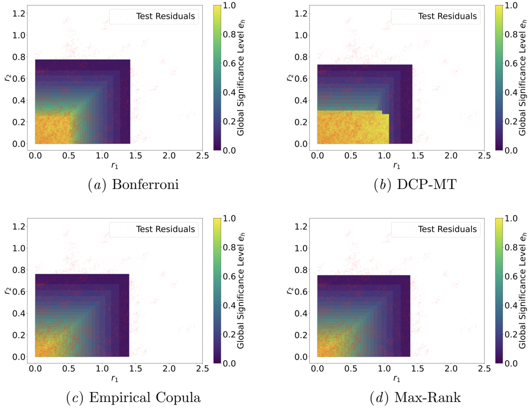
Figure 9: Multi-tests methods' partition of the residual space for the synthetic data set with e \sim \mathcal{N}(\mathbf{0}, \boldsymbol{\sigma}) , and \sigma = 0.5 averaged over 20 repetitions.
