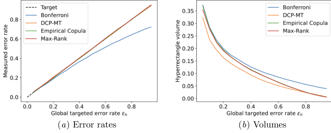
Figure 1: Multi-tests methods' mean error rates and volumes for the synthetic data set with e \sim [\mathcal{U}(-1, 1), \chi_2^2]^\top over 20 repetitions.
