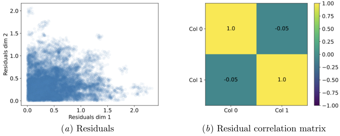
Figure 5: Underlying model's absolute residuals and their correlation for the synthetic data set with e \sim \mathcal{N}(\mathbf{0}, \sigma) , and \sigma = 0 .
