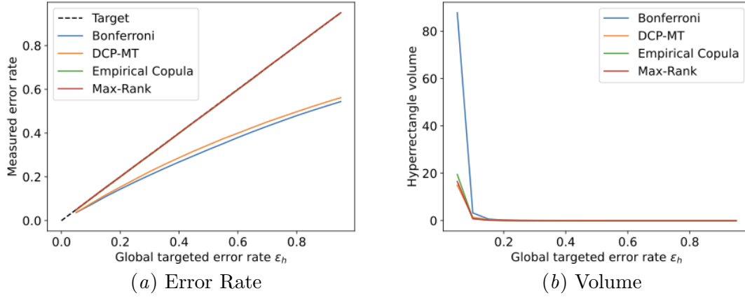
Figure 24: Multi-tests methods' mean error rates and volumes for the rf2 (Tsoumakas et al., 2011) data set.
