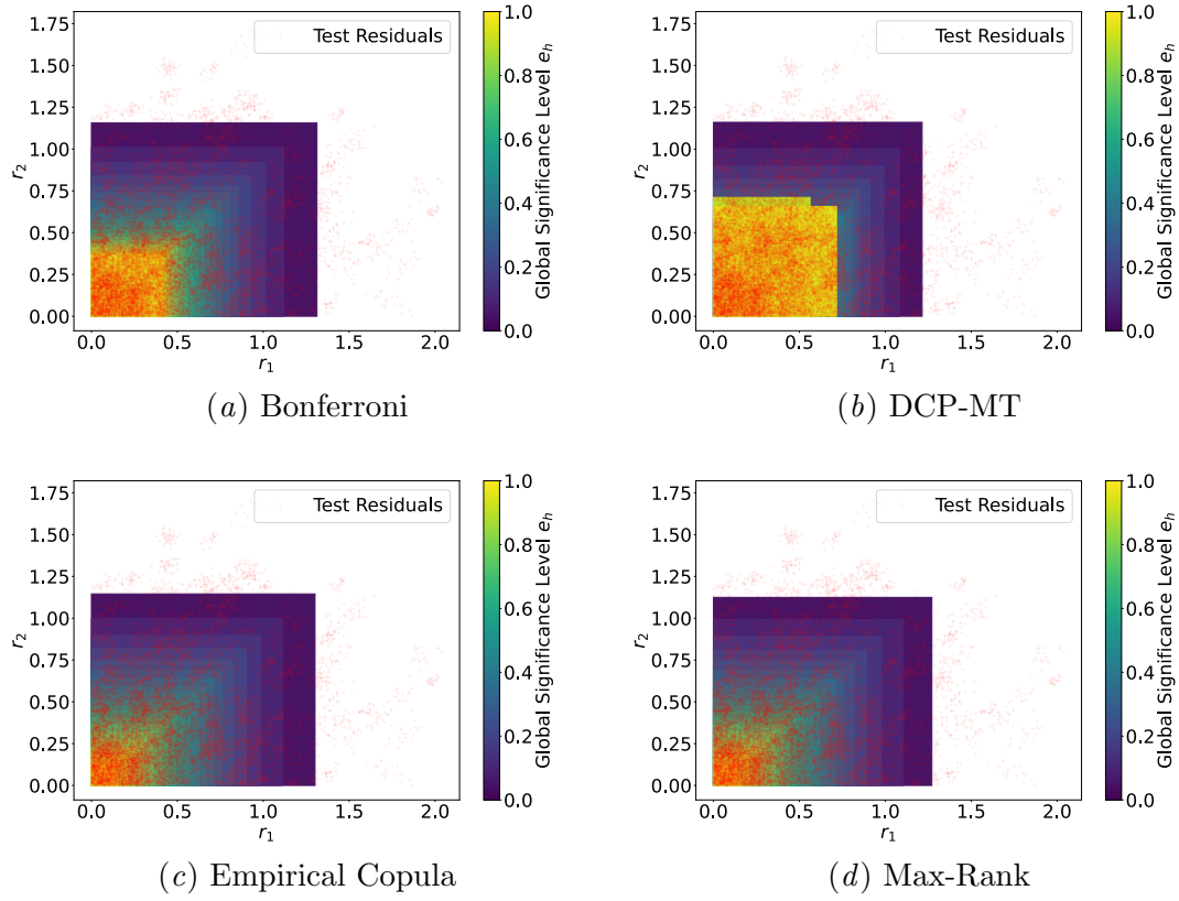
Figure 15: Multi-tests methods' partition of the residual space for the synthetic data set with e \sim \mathcal{N}(\mathbf{0}, \sigma) , and \sigma = -0.5 averaged over 20 repetitions.
