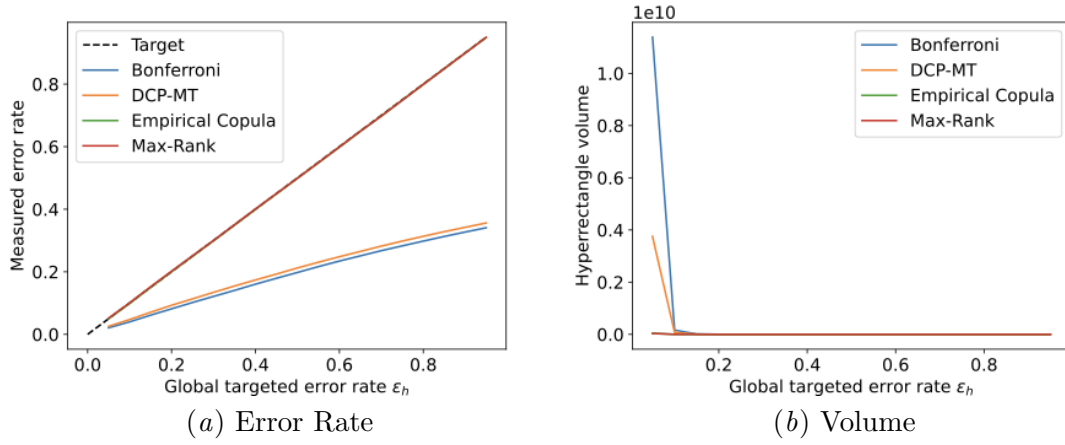
Figure 26: Multi-tests methods' mean error rates and volumes for the scm1d (Tsoumakas et al., 2011) data set.
