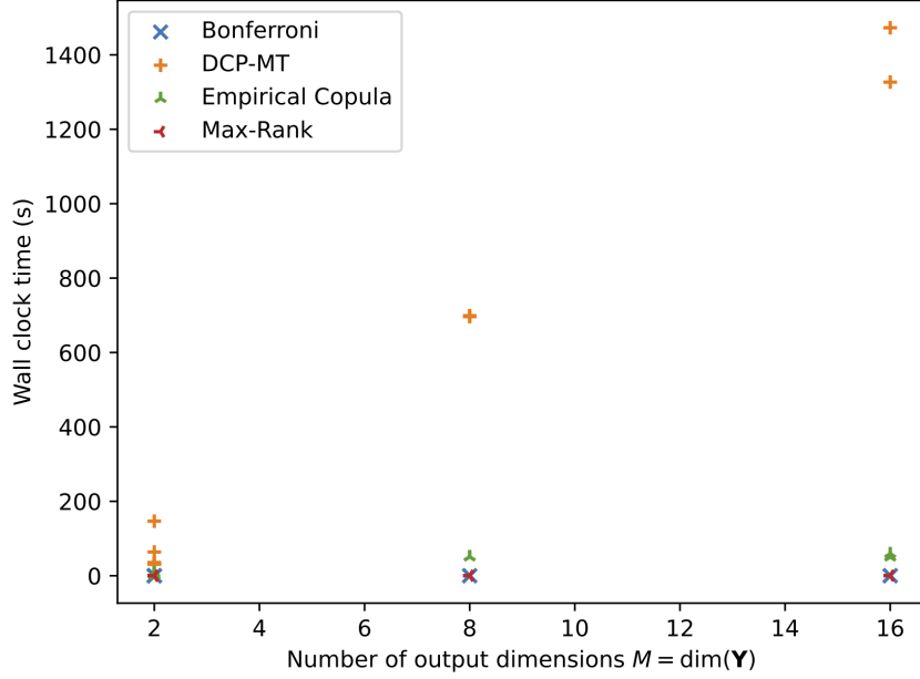
Figure 30: Total wall time in seconds across all experiments for multi-tests methods as a function of the number of dimensions in the label space M = \dim(\mathbf{Y}) .
