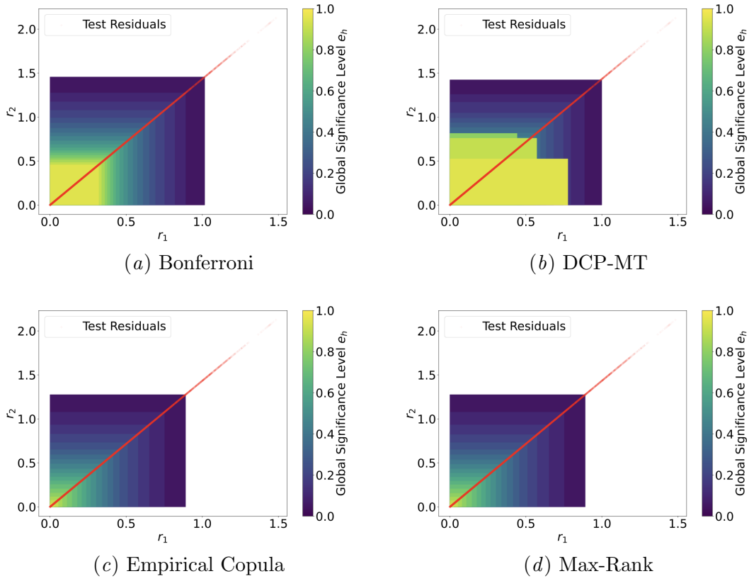
Figure 12: Multi-tests methods' partition of the residual space for the synthetic data set with e \sim \mathcal{N}(\mathbf{0}, \sigma) , and \sigma = 1 averaged over 20 repetitions.
