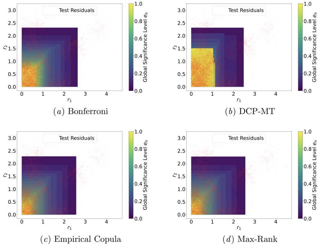
Figure 21: Multi-tests methods' partition of the residual space for the music origin (Zhou et al., 2014) data set.
