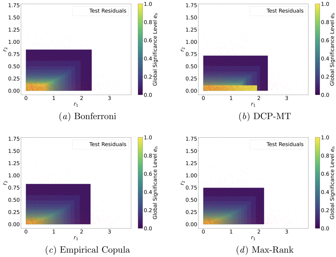
Figure 18: Multi-tests methods' partition of the residual space for the diabetes ( Efron et al., 2004 ) data set.
