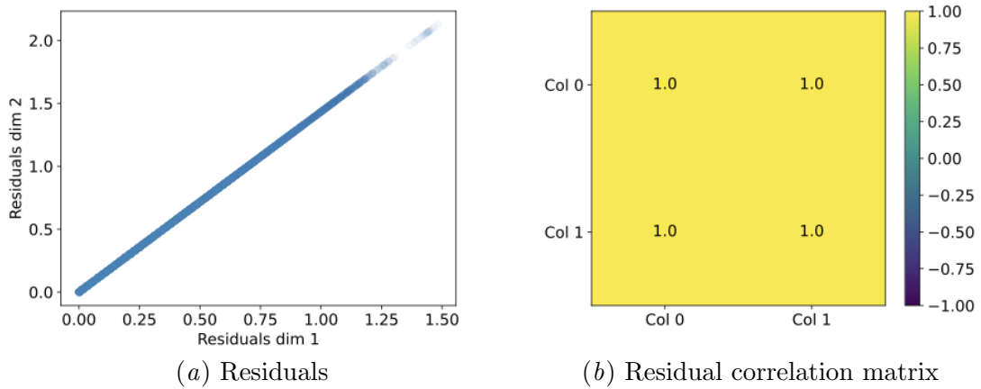
Figure 11: Underlying model's absolute residuals and their correlation for the synthetic data set with e \sim \mathcal{N}(\mathbf{0}, \sigma) , and \sigma = 1 .
