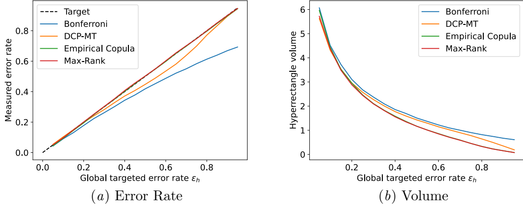
Figure 13: Multi-tests methods' mean error rates and volumes for the synthetic data set with e \sim \mathcal{N}(\mathbf{0}, \sigma) , and \sigma = -0.5 .
