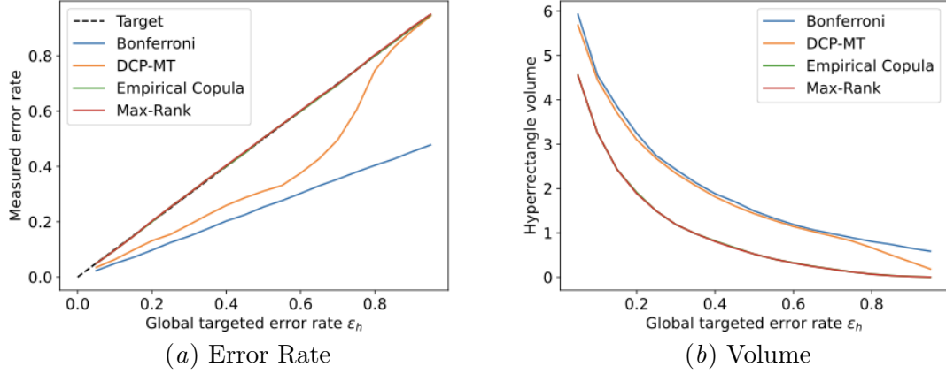
Figure 10: Multi-tests methods' mean error rates and volumes for the synthetic data set with e \sim \mathcal{N}(\mathbf{0}, \sigma) , and \sigma = 1 .
