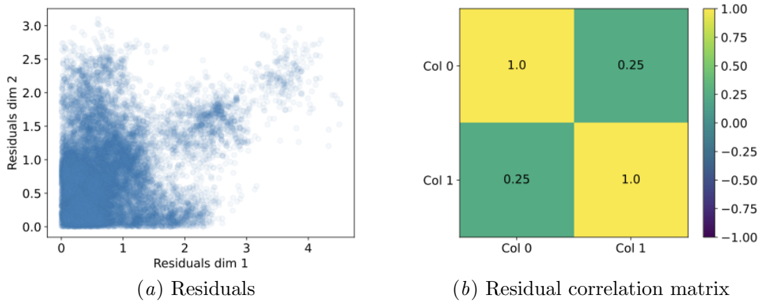
Figure 20: Underlying model's absolute residuals and their correlation for the music origin (Zhou et al., 2014) data set.
