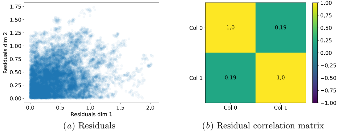
Figure 14: Underlying model's absolute residuals and their correlation for the synthetic data set with e \sim \mathcal{N}(\mathbf{0}, \sigma) , and \sigma = -0.5 .
