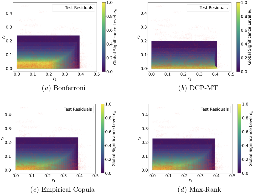
Figure 3: Multi-tests methods' partition of the residual space for the synthetic data set with e \sim [\mathcal{U}(-1, 1), \chi_2^2]^\top averaged over 20 repetitions.
