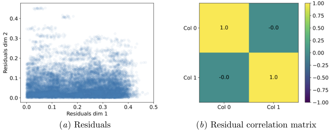
Figure 2: Underlying model's absolute residuals and their correlation for the synthetic data set with e \sim [\mathcal{U}(-1, 1), \chi_2^2]^\top .
