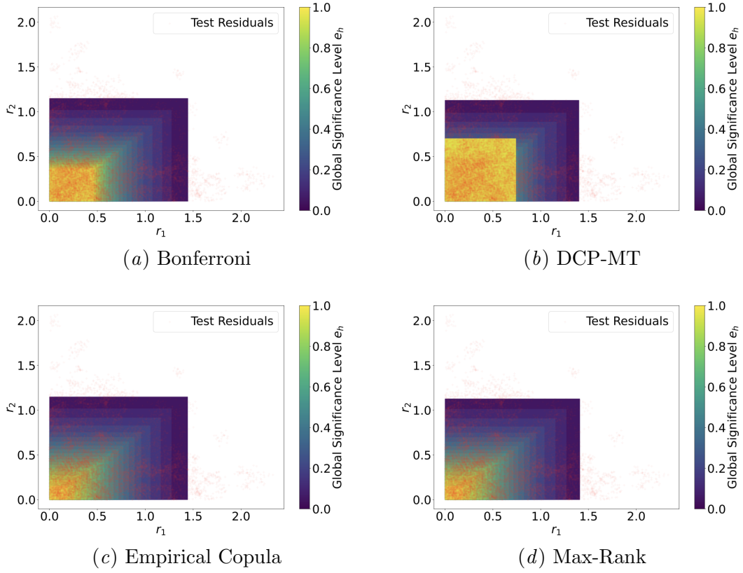
Figure 6: Multi-tests methods' partition of the residual space for the synthetic data set with e \sim \mathcal{N}(\mathbf{0}, \boldsymbol{\sigma}) , and \sigma = 0 averaged over 20 repetitions.
