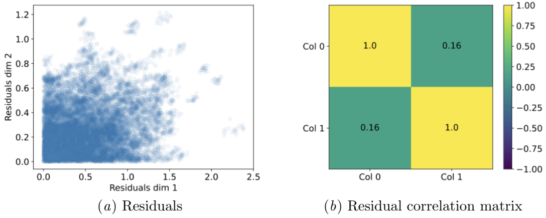
Figure 8: Underlying model's absolute residuals and their correlation for the synthetic data set with e \sim \mathcal{N}(\mathbf{0}, \sigma) , and \sigma = 0.5 .
