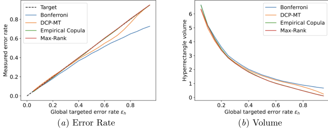
Figure 4: Multi-tests methods' mean error rates and volumes for the synthetic data set with e \sim \mathcal{N}(\mathbf{0}, \sigma) , and \sigma = 0 .
