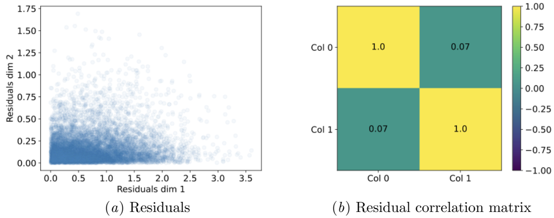
Figure 17: Underlying model's absolute residuals and their correlation for the diabetes (Efron et al., 2004) data set.
