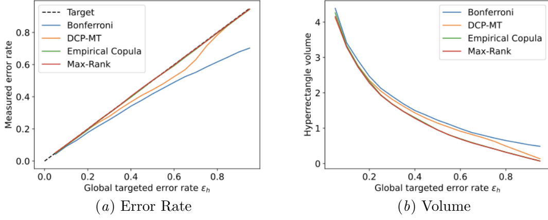
Figure 7: Multi-tests methods' mean error rates and volumes for the synthetic data set with e \sim \mathcal{N}(\mathbf{0}, \sigma) , and \sigma = 0.5 .
