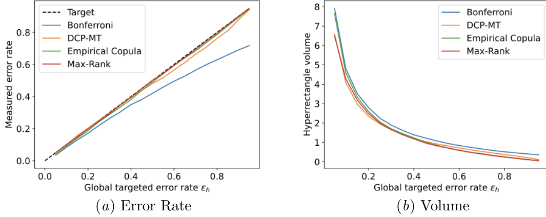
Figure 16: Multi-tests methods' mean error rates and volumes for the diabetes (Efron et al., 2004) data set.
