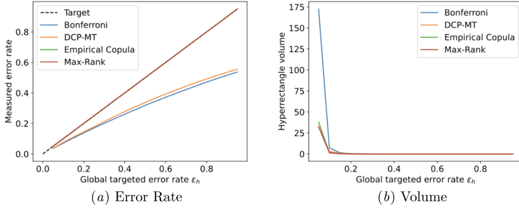
Figure 22: Multi-tests methods' mean error rates and volumes for the rf1 (Tsoumakas et al., 2011) data set.
